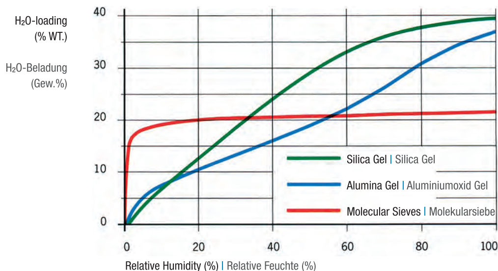
Water adsorption of different drying agents
